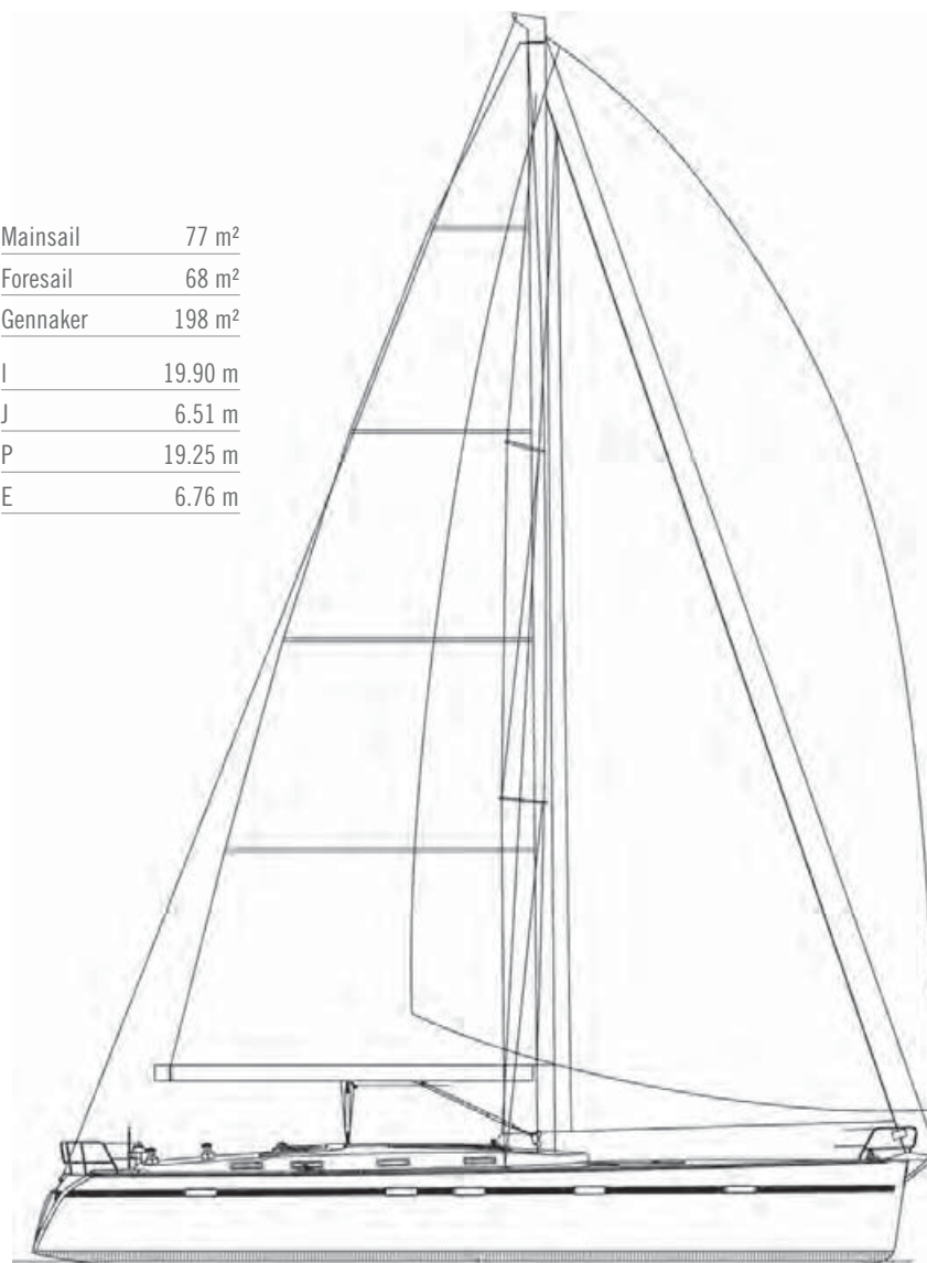
Sail plan
